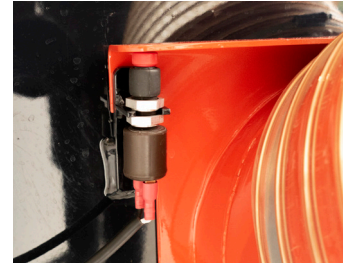
Safety sensor on fan housing shuts off engine during maintenance work.
